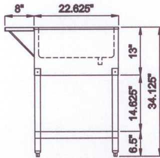
SECTIONAL VIEW
