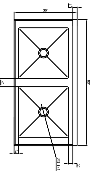
PLAN VIEW
